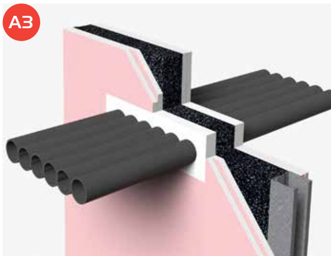
FZ100 Fire Safe Zone and row of combustable pipes
